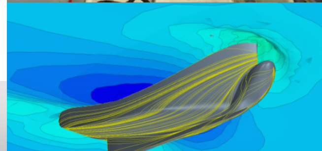
Bulbous-bow design for a west coast fishing vessel
